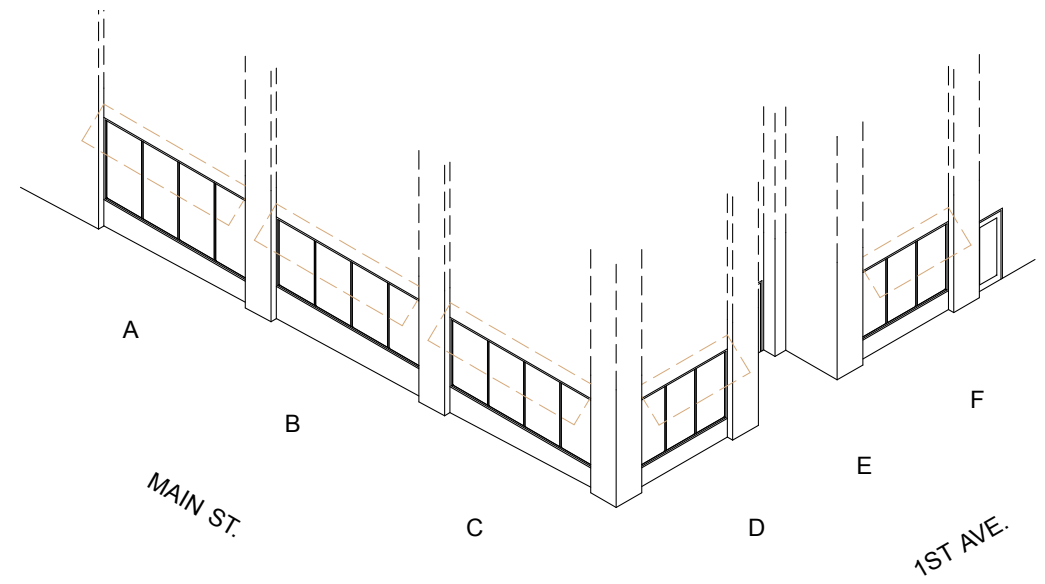
3 ISOMETRIC NOT TO SCALE
